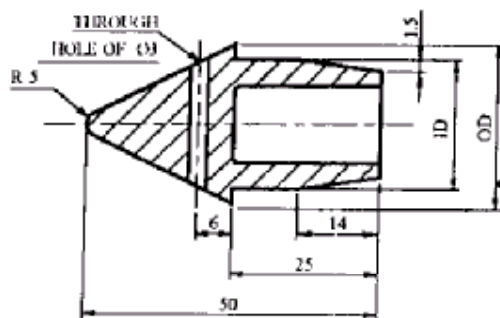
FIG. 2 TYPICAL DRAWING OF CAP FOR TUBE END
